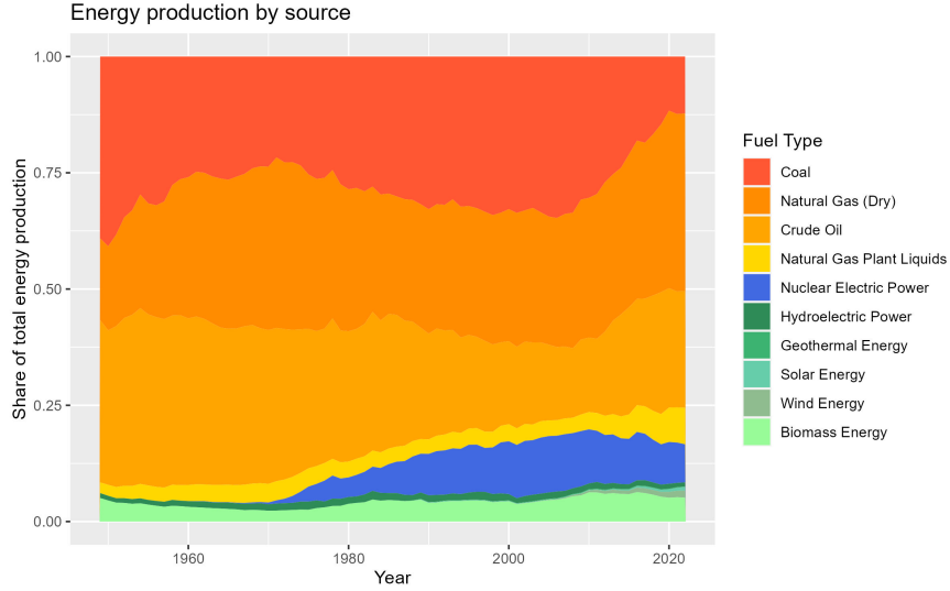
Figure 2: Shares of energy production in detail
